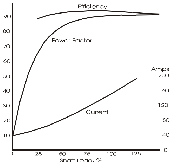
Toshiba 90KW 4pole motor.
